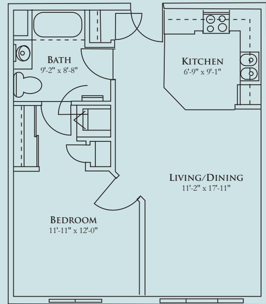
ONE BEDROOM UNIT PLAN — TYPE B
